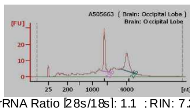
Fig. 2 Total RNA was analyzed by Agilent bio-chip
