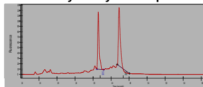
Fig. 2 Total RNA was analyzed by Agilent bio-chip
