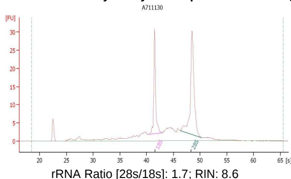
Fig. 2 Total RNA was analyzed by Agilent bio-chip
