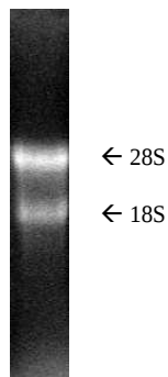
Fig. 1 Total RNA was analyzed by electrophoresis on 1% agarose gel
