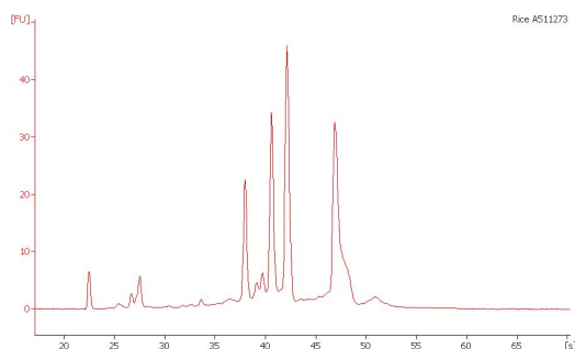
Fig. 2 Total RNA was analyzed by Agilent bio-chip
