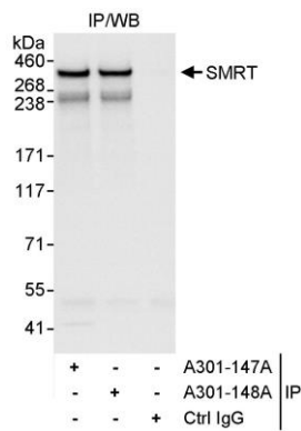
Detection of human SMRT by western blot of immunoprecipitates. Samples: Whole cell lysate (1 mg for IP, 20% of IP loaded) from HeLa cells. Antibodies: Affinity purified rabbit anti-SMRT antibody A301-148A used for IP at 3 µg/mg lysate. SMRT was also immunoprecipitated by rabbit anti-SMRT antibody A301-147, which recognizes an upstream epitope. For blotting immunoprecipitated SMRT, A301-147A was used at 1 µg/ml. Detection: Chemiluminescence with an exposure time of 1 second.
