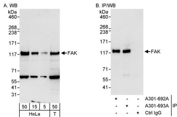
Detection of human FAK by western blot and immunoprecipitation. Samples: Whole cell lysate from HeLa (5, 15 and 50 µg for WB; 1 mg for IP, 20% of IP loaded) and HEK293T (T; 50 µg) cells. Antibodies: Affinity purified rabbit anti-FAK antibody A301-693A used for WB at 0.04 µg/ml (A) and 1 µg/ml (B) and used for IP at 3 µg/mg lysate. FAK was also immunoprecipitated by rabbit anti-FAK antibody A301-692A, which recognizes an upstream epitope. Detection: Chemiluminescence with exposure times of 30 seconds (A) and 3 seconds (B).
