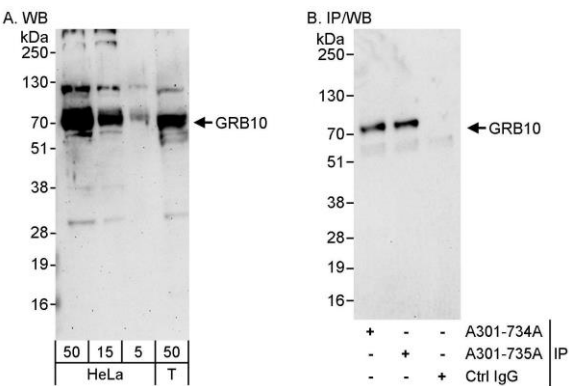
Detection of human GRB10 by western blot and immunoprecipitation. Samples: Whole cell lysate from HeLa (5, 15 and 50 µg for WB; 1 mg for IP, 20% of IP loaded) and HEK293T (T; 50 µg) cells. Antibodies: Affinity purified rabbit anti-GRB10 antibody A301-734A used for WB at 0.1 µg/ml (A) and 0.4 µg/ml (B) and used for IP at 3 µg/mg lysate. GRB10 was also immunoprecipitated by rabbit anti-GRB10 antibody A301-735A, which recognizes a downstream epitope. Detection: Chemiluminescence with exposure times of 3 minutes (A) and 30 seconds (B).
