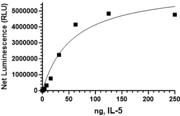
IL-5:IL-5Ra Binding Activity
