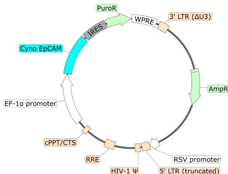
Figure 1. Schematic of the lenti-vector used to generate the Cyno EpCAM Lentivirus.
