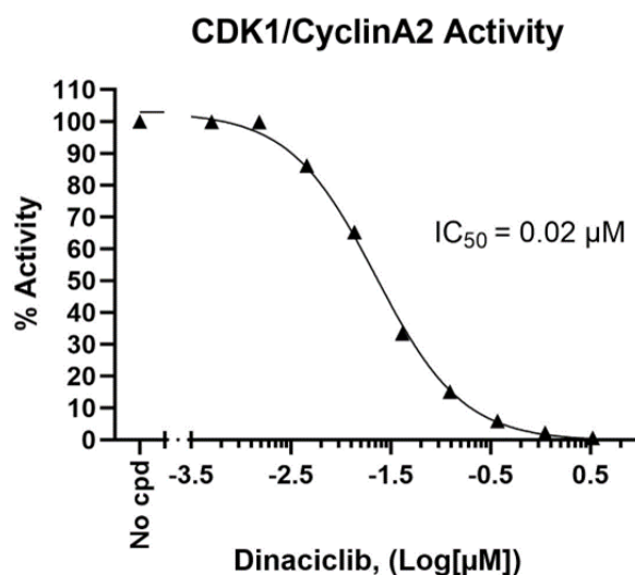
Figure 1: Inhibition of CDK1/CyclinA2 kinase activity by Dinaciclib.
