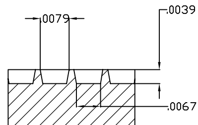
SECTION X-X
