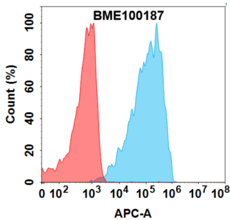
Figure 1. Flow cytometry analysis with 1µg/mL Anti-GPRC5D(LM305 biosimilar) mAb (BME100187) on Expi293 cells transfected with Human GPRC5D protein (Blue histogram) or Expi293 transfected with irrelevant protein (Red histogram).
