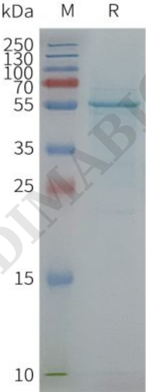
Figure2. Human TMCC3-Nanodisc, Flag Tag on SDS-PAGE
