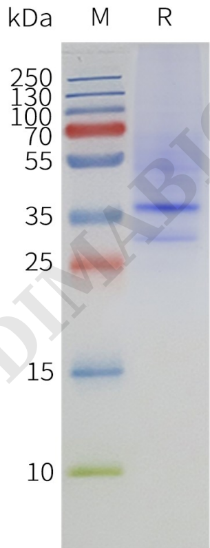
Figure 2. Human MTR1A-Strep-Nanodisc, C-Flag&Strep Tag on SDS-PAGE
