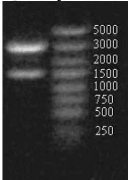
RES:HindIII
