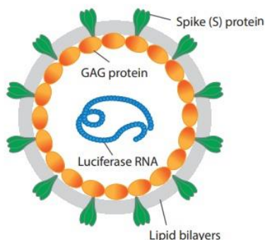
Figure 1. Illustration of the replication-deficient MLV particle pseudotyped with SARS-CoV Spike protein
