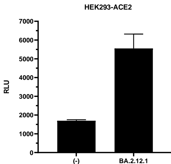
Figure 2. Pseudoviral Particle (PP) Infection assays (SARS-CoV-2 Omicron BA.2.12.1 variant pseudoviral particles on HEK293-ACE2 cells)
