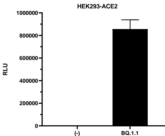
Figure 2. Pseudoviral Particle (PP) Infection assays (SARS-CoV-2 Omicron BQ.1.1 variant pseudoviral particles on HEK293-ACE2 cells; Luminescence plate reader: BioTek Synergy 2)
