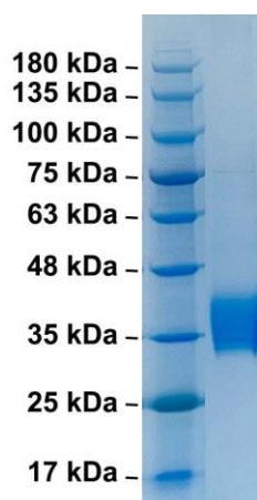
SDS-PAGE: purified recombinant spike RBD protein of SARS-CoV-2 Omicron XBB variant
