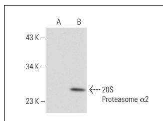
20S Proteasome \alpha 2 (MCP21): sc-58413. Western blot analysis of 20S Proteasome \alpha 2 expression in non-transfected: sc-117752 (A) and human 20S Proteasome \alpha 2 transfected: sc-116165 (B) 293T whole cell lysates.
