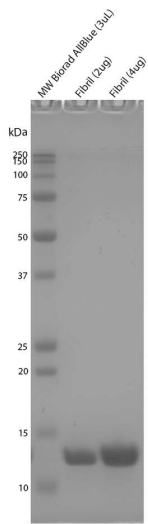
SDS-PAGE of Tau dGAE AD-mimic fibrils (SPR-502) on a 12% Tris-Glycine Gel.
