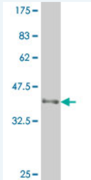
Western Blot detection against Immunogen (40.3 KDa) .
