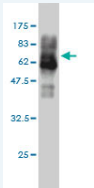
Western Blot detection against Immunogen (77.66 KDa) .
