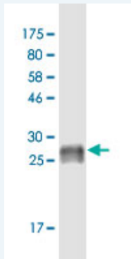
Western Blot detection against Immunogen (22.11 kDa) .
