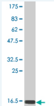
Western Blot detection against Immunogen (17.7 kDa)
