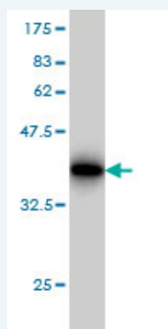
Western Blot detection against Immunogen (32.89 KDa) .
