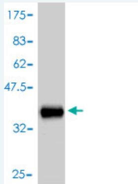
Western Blot detection against Immunogen (39.53 KDa) .
